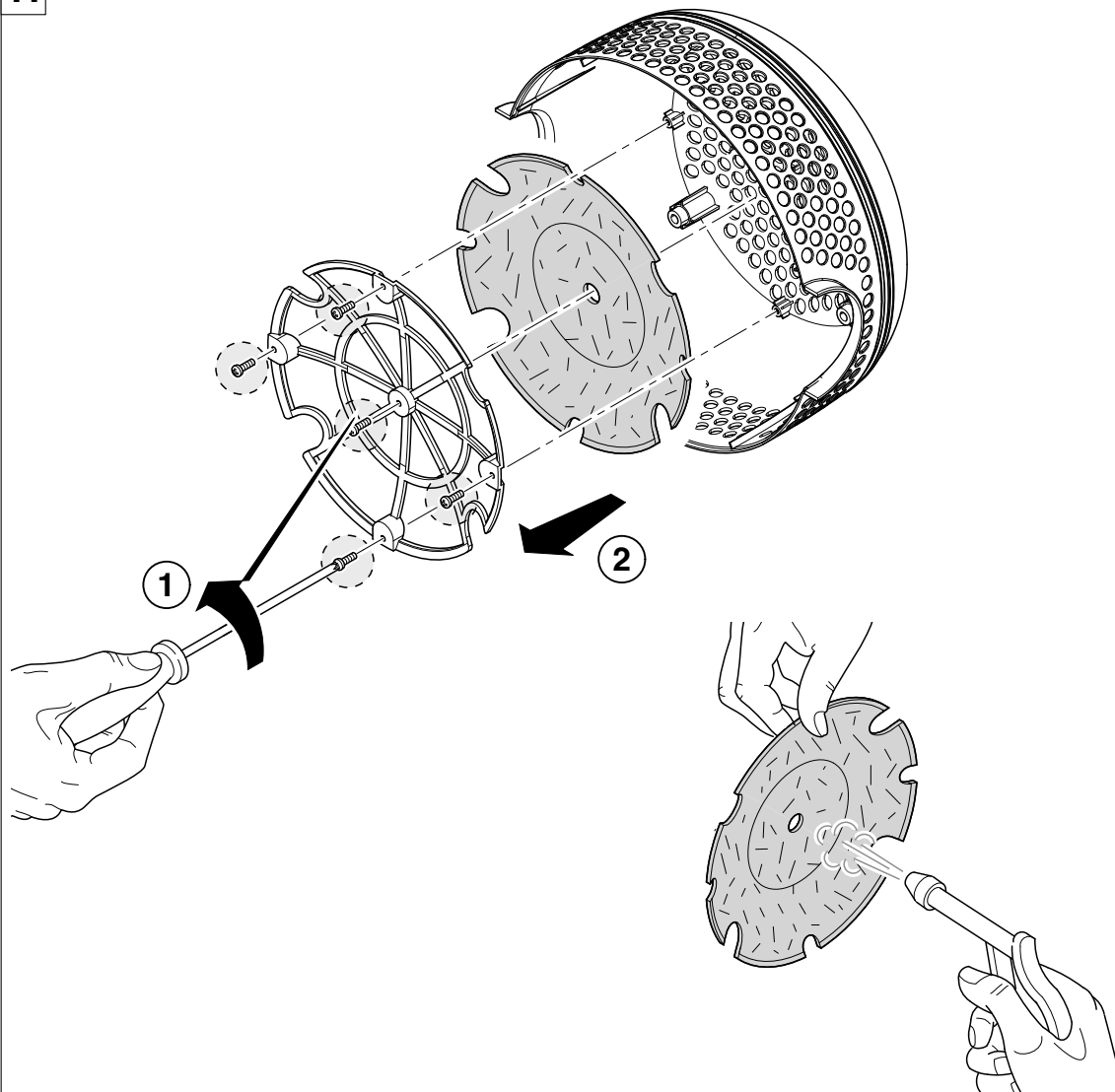
Cleaning the filters - Fig. 14
