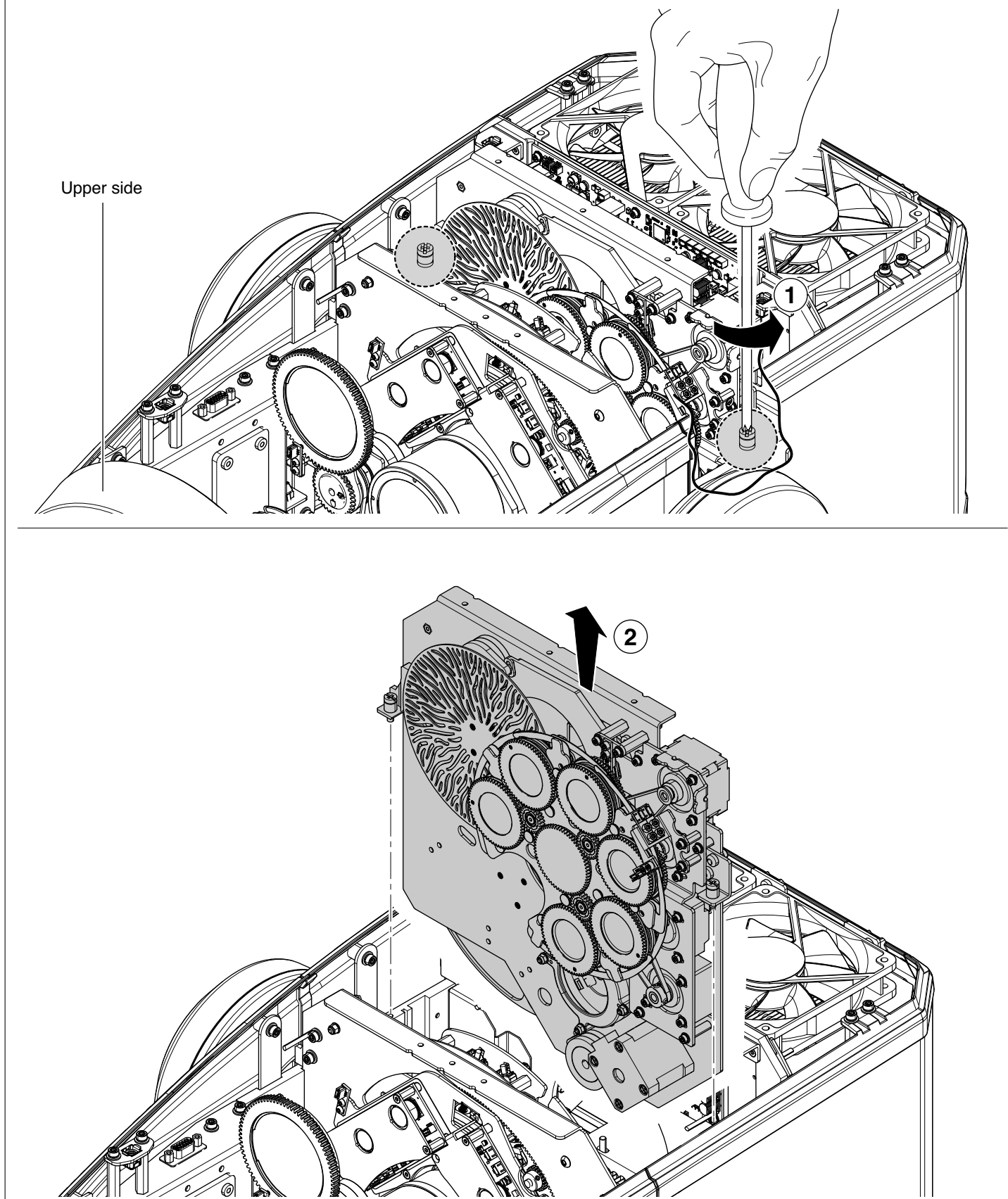
Extraction of the effect modules - Fig. 15.
