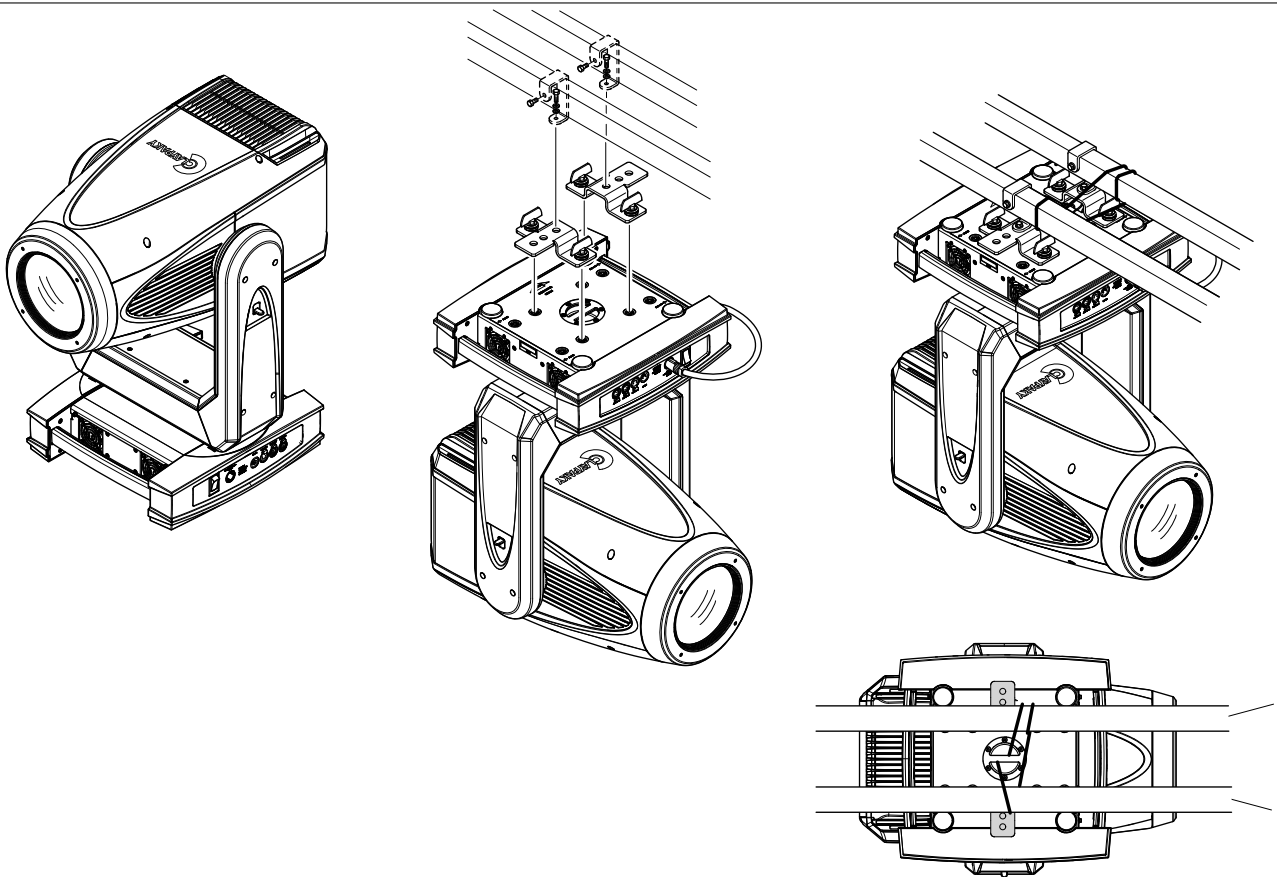
Installing the projector - Fig. 4
