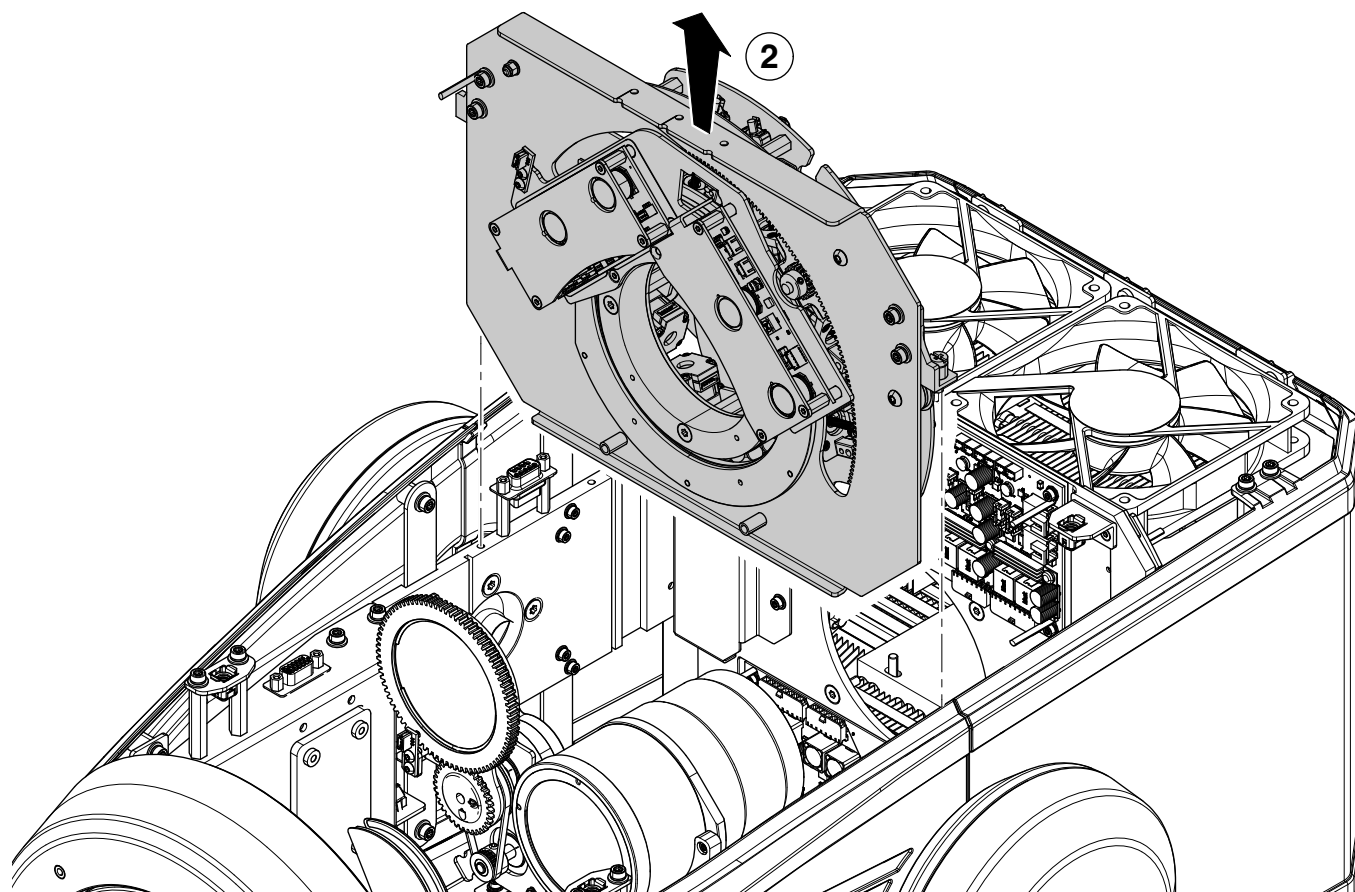
Extraction of the effect modules - Fig. 16.
