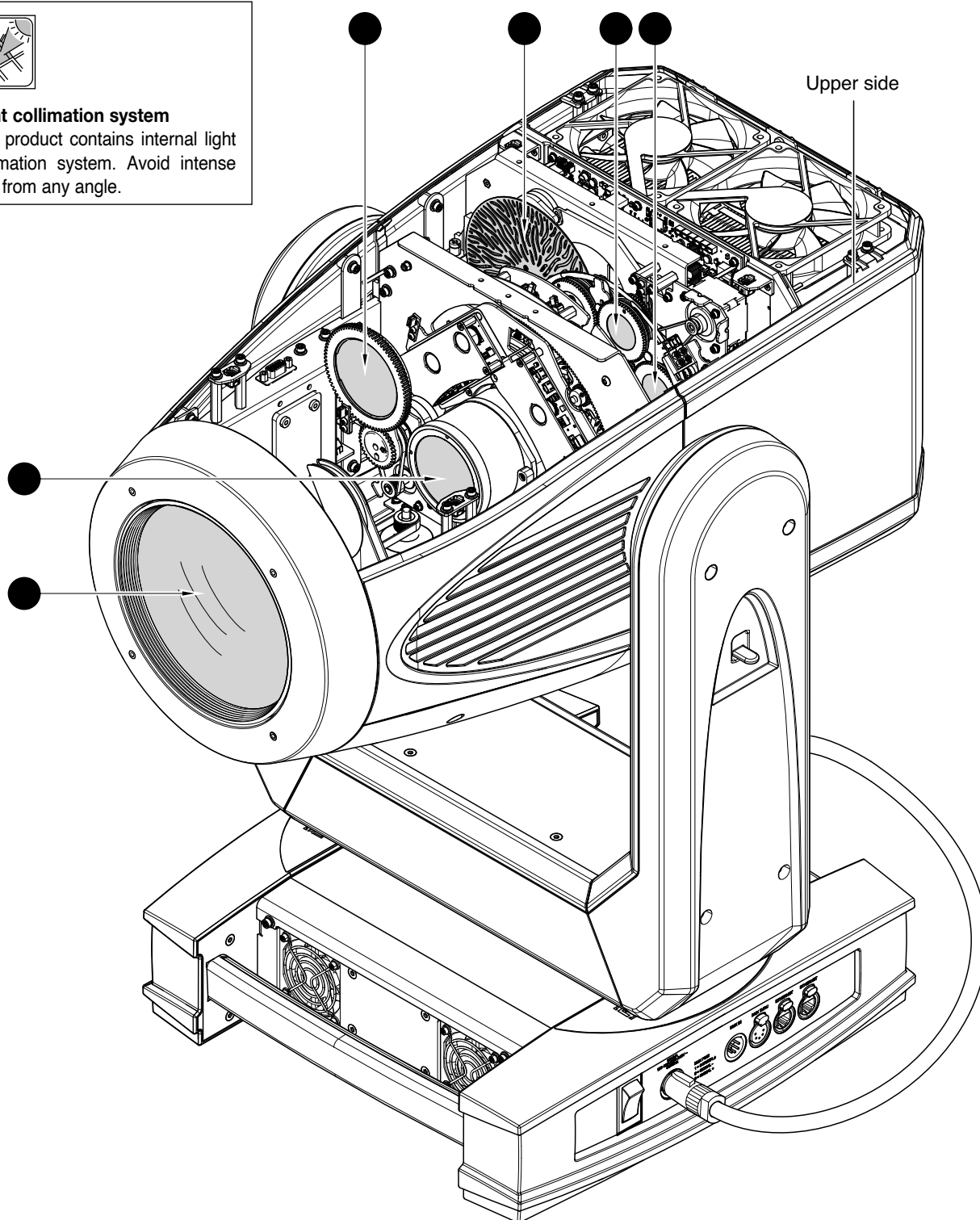
Periodical cleaning - Fig. 13
