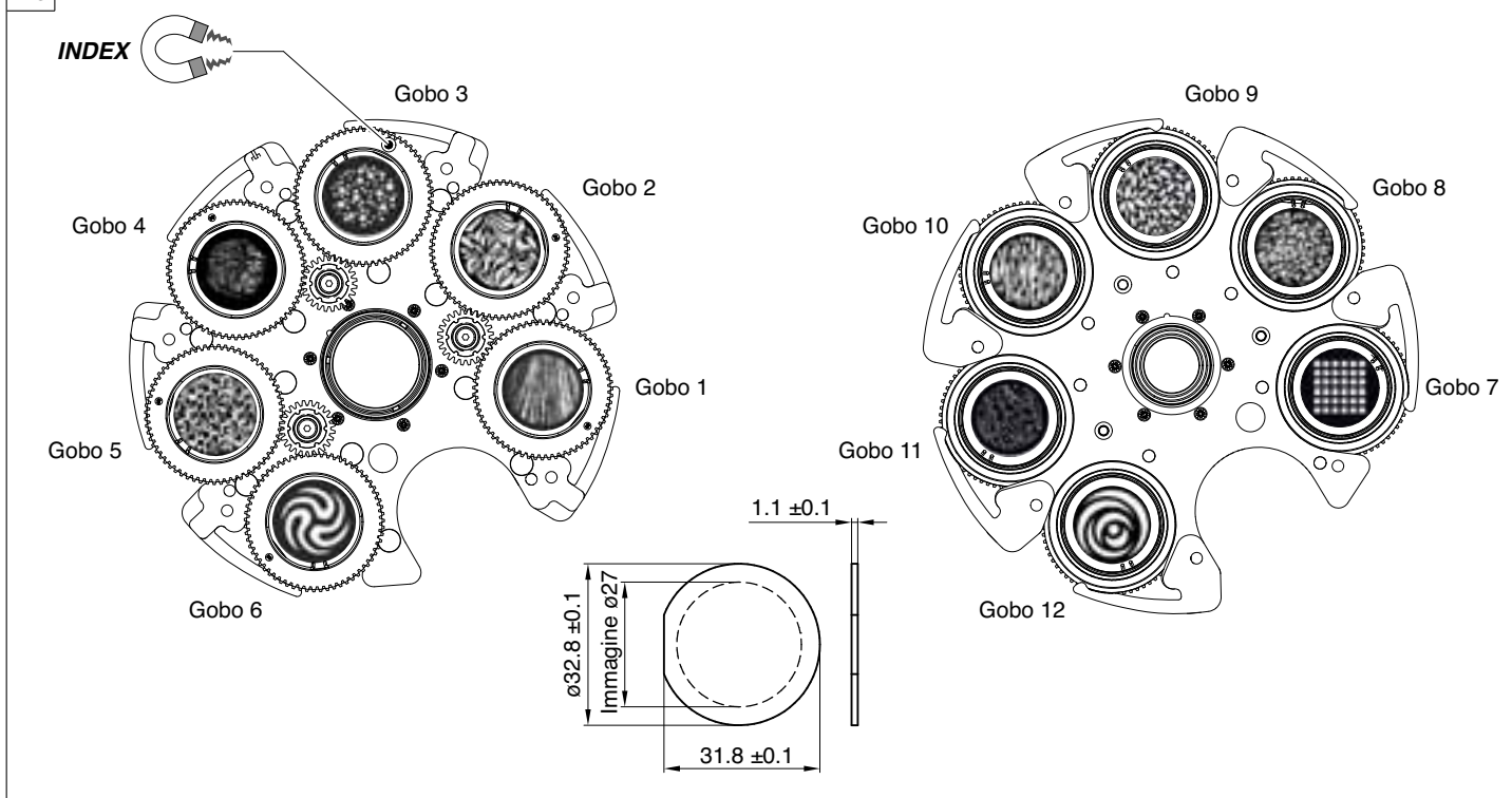
Replacing rotating gobos (max 27 mm image – thickness 1.1 mm) - Fig. 19
