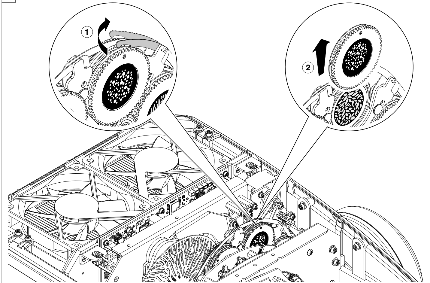
Bearing group replacement - Fig. 18
