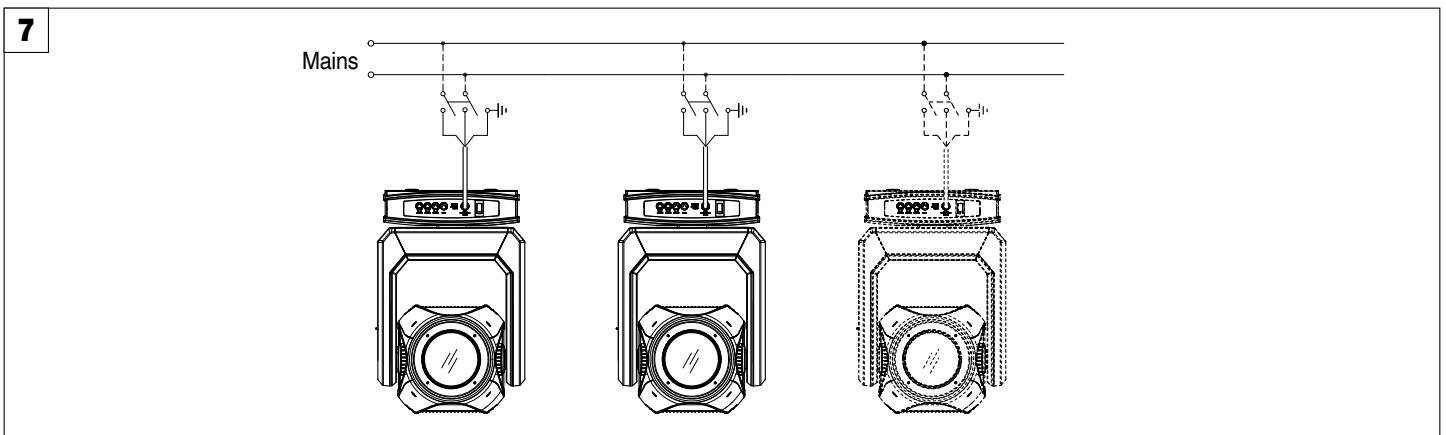
Connecting to the mains supply - Fig. 7
