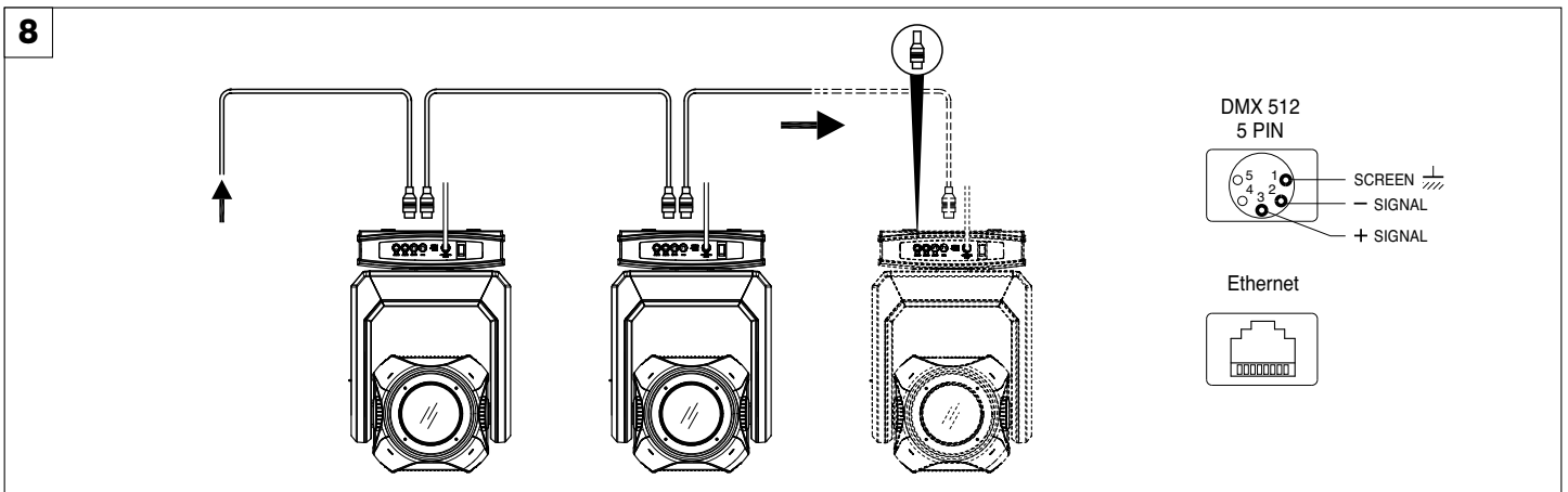
Connecting to the control signal line (DMX) - Fig. 8
