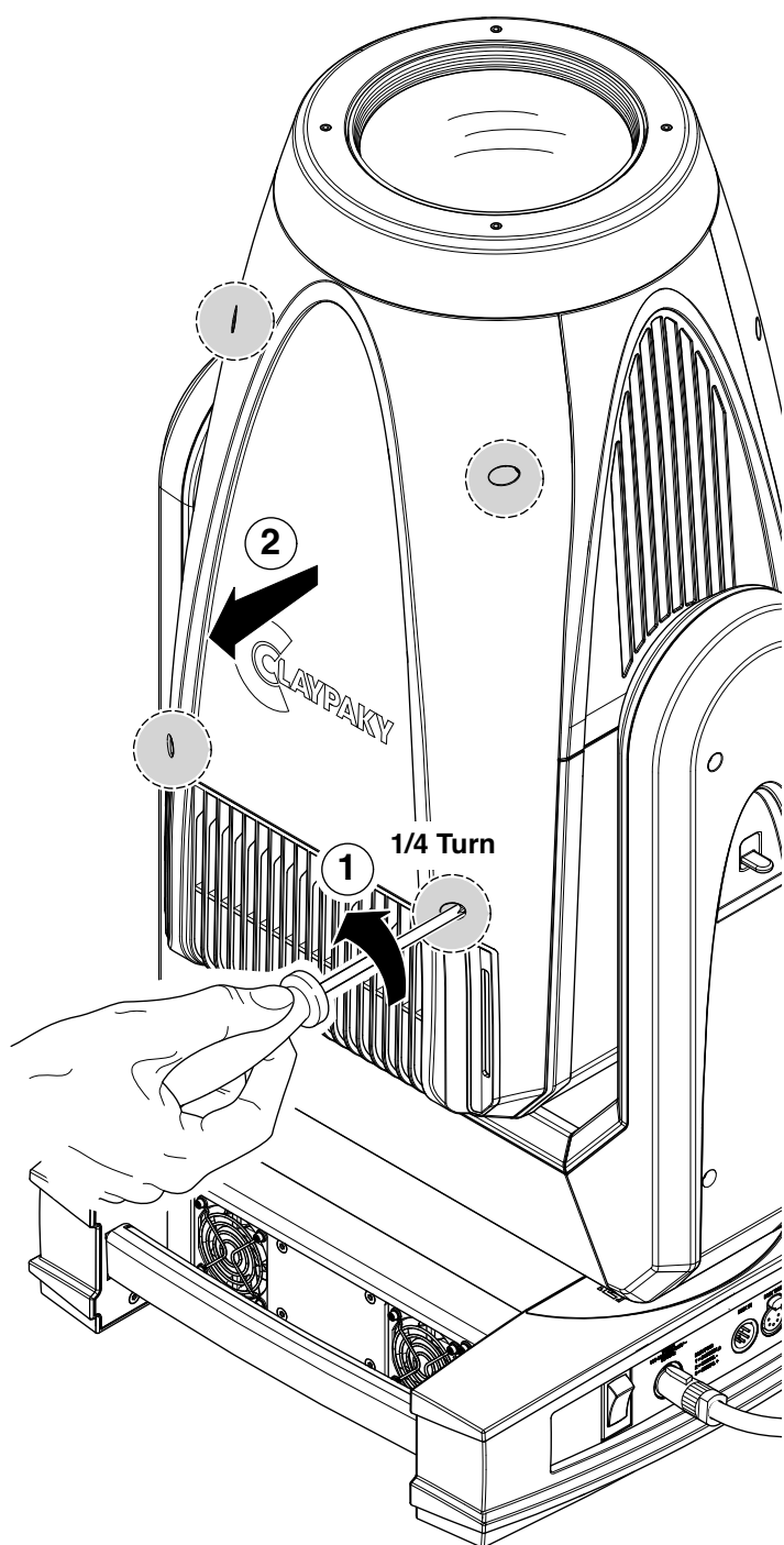
Cleaning of the grids - Fig. 17
